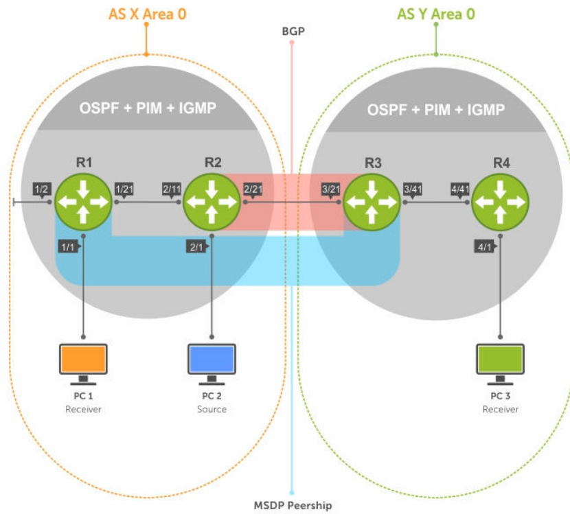
Figure 74. Multicast Source Discovery Protocol (MSDP)
